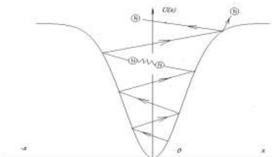
Fig.7. Oscillation of Nitrogen molecule in potential well of catalyst.
