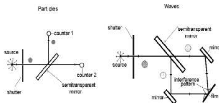
Fig.1. Experiments with individual photons on semitransparent mirror.
