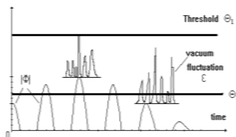
Fig.4. Quantum measurements.
