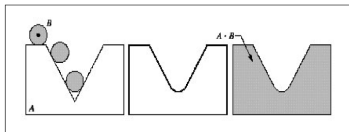
Figure 2.9: Illustration of Binary Closing Process [13]
