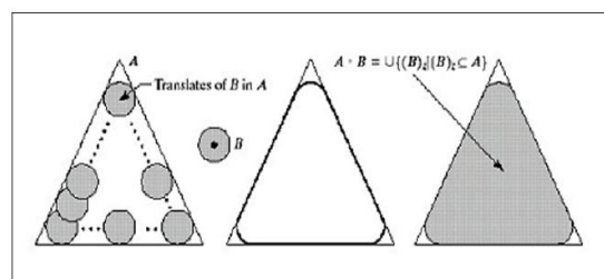
Figure 2.7: Illustration of Binary Opening Process [13]
