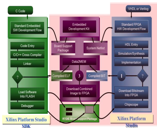
Figure4: Embedded Development Kit Design Flow
