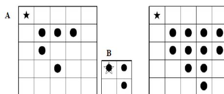
Figure 2.3: Illustration of Binary Dilation on Digital Setting
